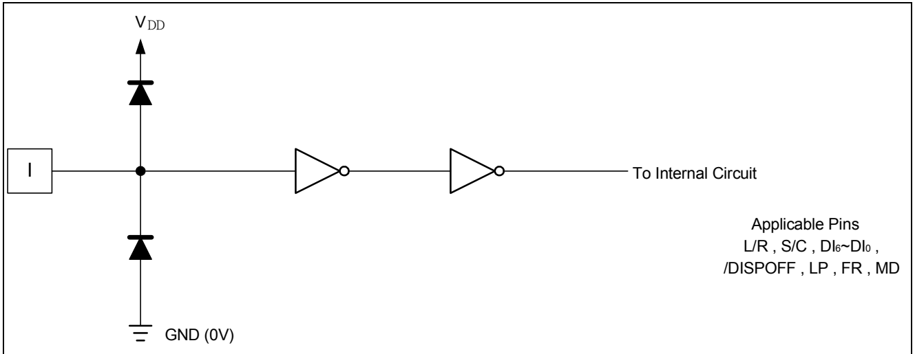
Figure 6-1 Input Circuit (1)
