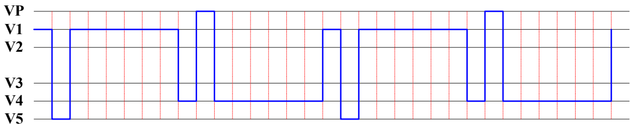
FIGURE 15-2 LCD Common Waveform
