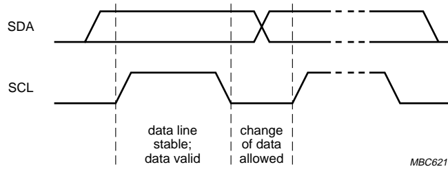
Fig.20 Bit transfer.
