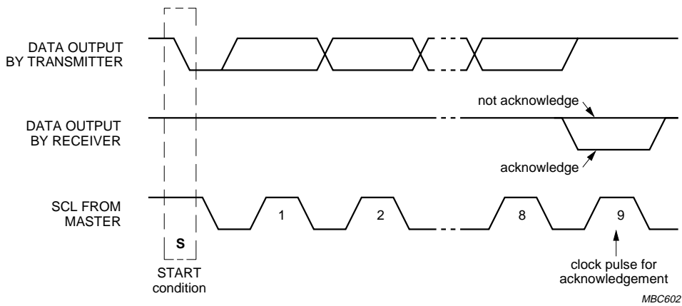
Fig.22 Acknowledgement on the I 2 C-bus.
