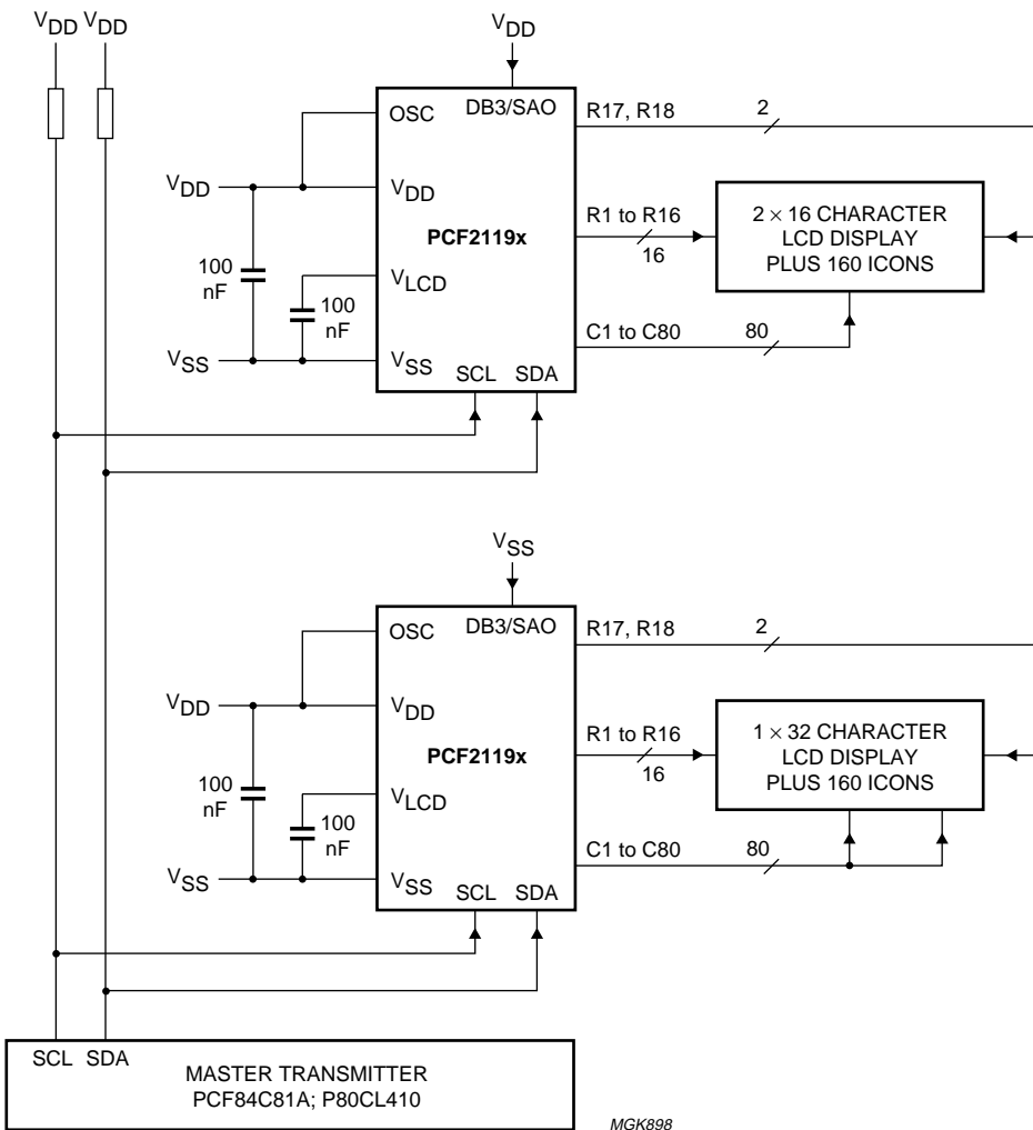
Fig.32 Application using I 2 C-bus interface.
