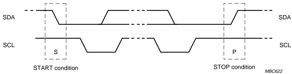
Fig.21 Definition of START and STOP conditions.
