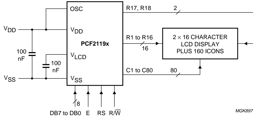
Fig.31 Typical application using parallel interface.
