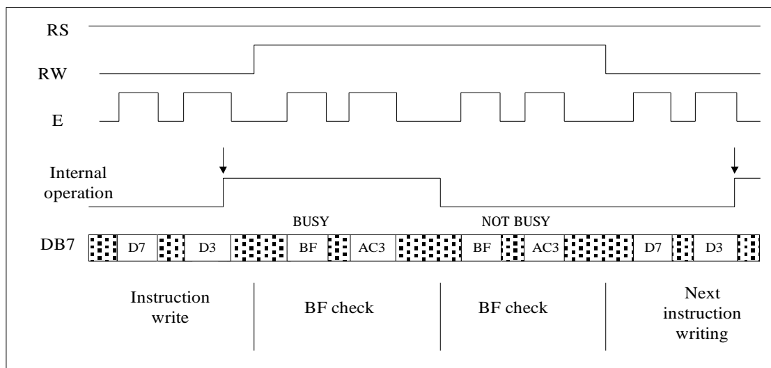
Fig.5. Example of 4-bit Bus Mode Timing Diagram
