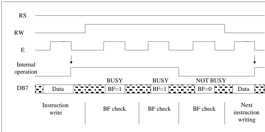
Fig.4. Example of 8-bit Bus Mode Timing Diagram
