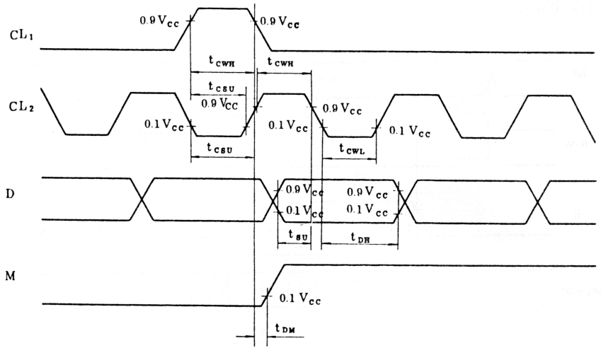
Fig. 3 Sending Data to Driver LSI HD44100H
