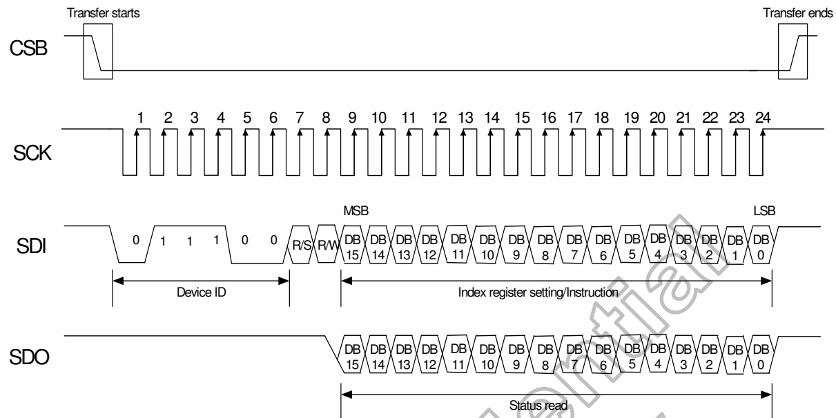
Figure 6. 1 SPI Timing
