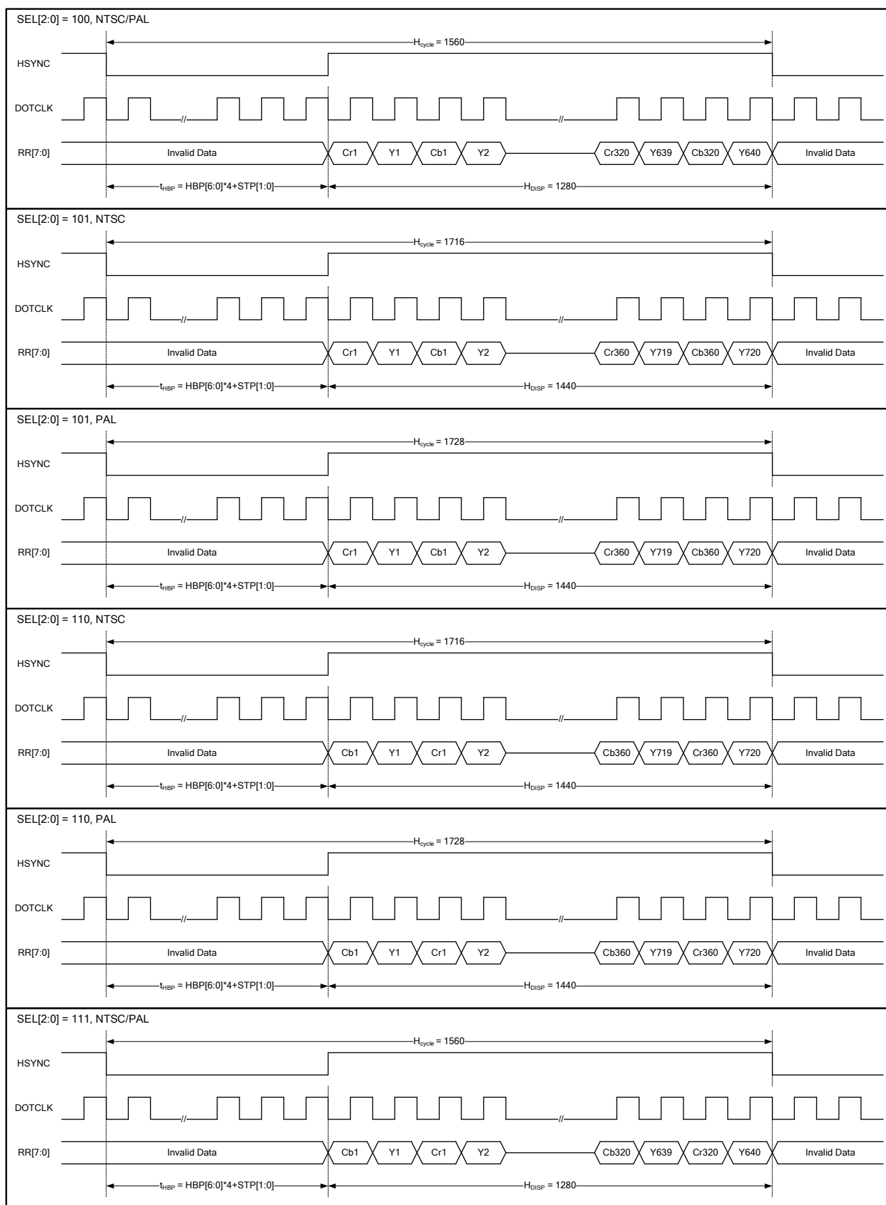
Figure13. 7 CCIR601 Horizontal Timing
