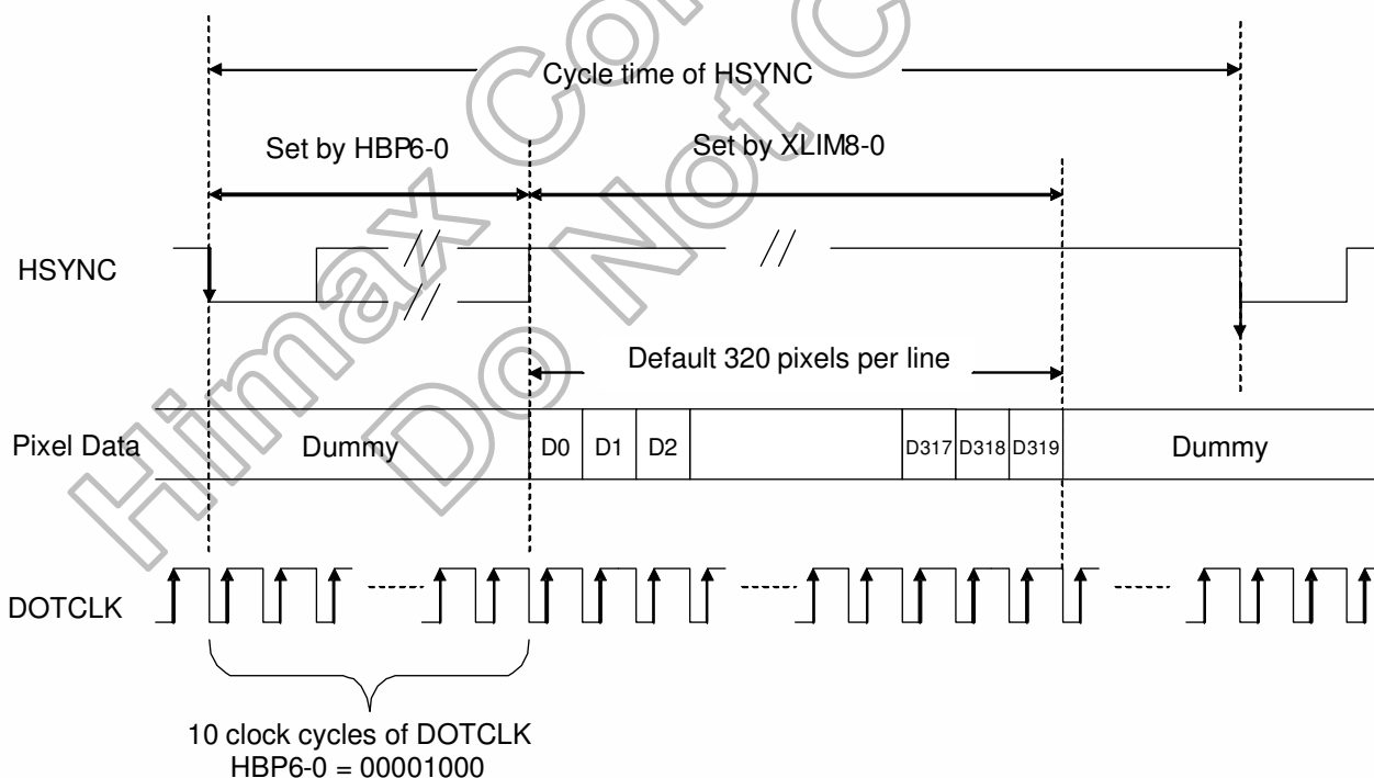
Figure 8. 18 No. of Clock Cycle of Clock
