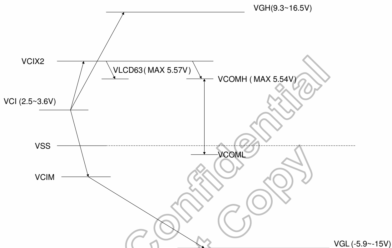
Figure 14. 1 LCD Driving Voltage Relationship
