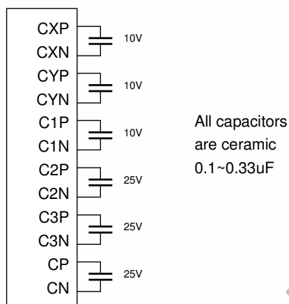
Figure 15.1 Booster Capacitors
