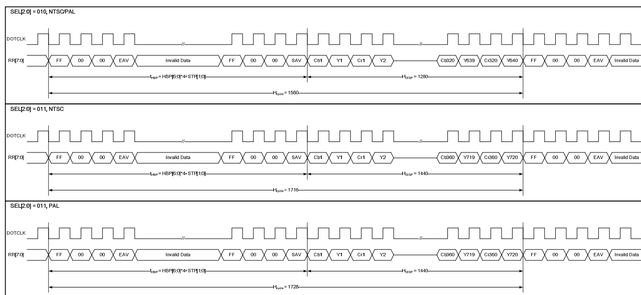
Figure13. 9 CCIR656 Horizontal Timing
