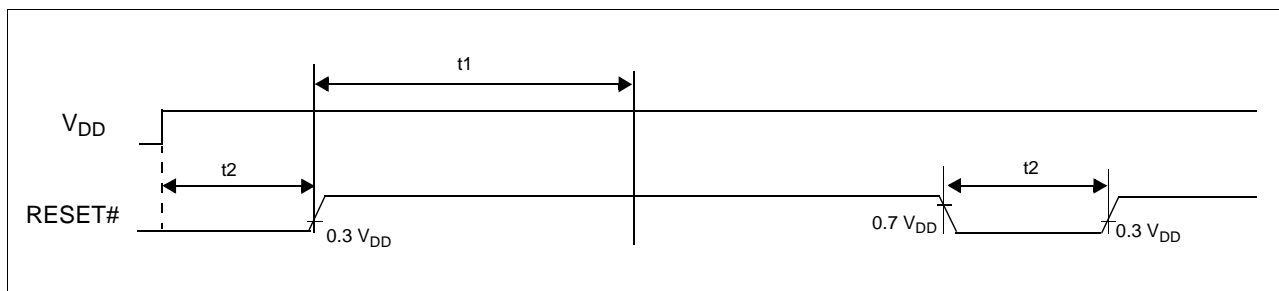
Figure 7-2 Reset Timing
