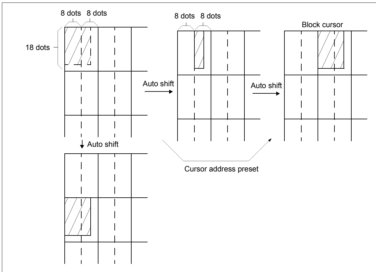
Figure 12-10 Cursor Movement
