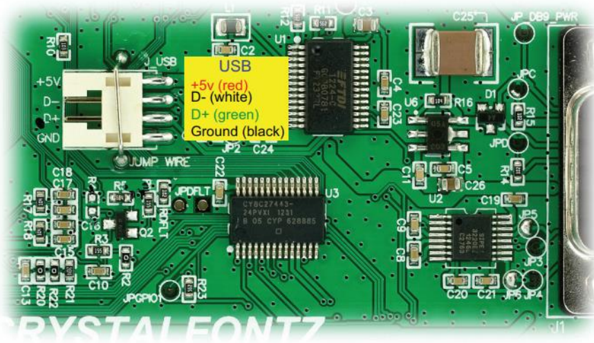
Figure 4. USB Connector Pins Labeled
