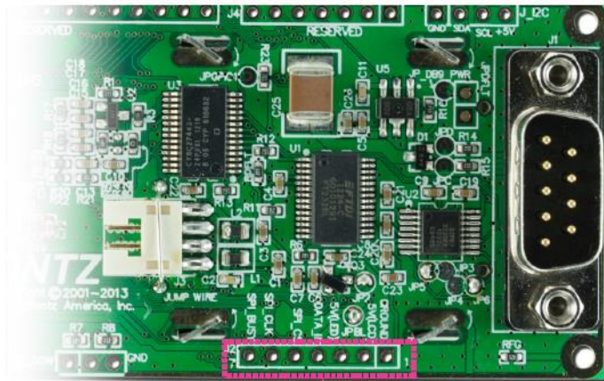
J2 7-Pin Expansion Port For LL Or LLi Interface
