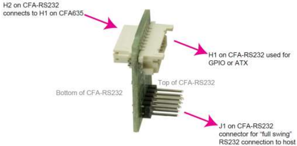
Figure 8. CFA-RS232 Level Translator
