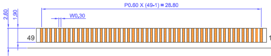
(A) FPC Pin Detail
