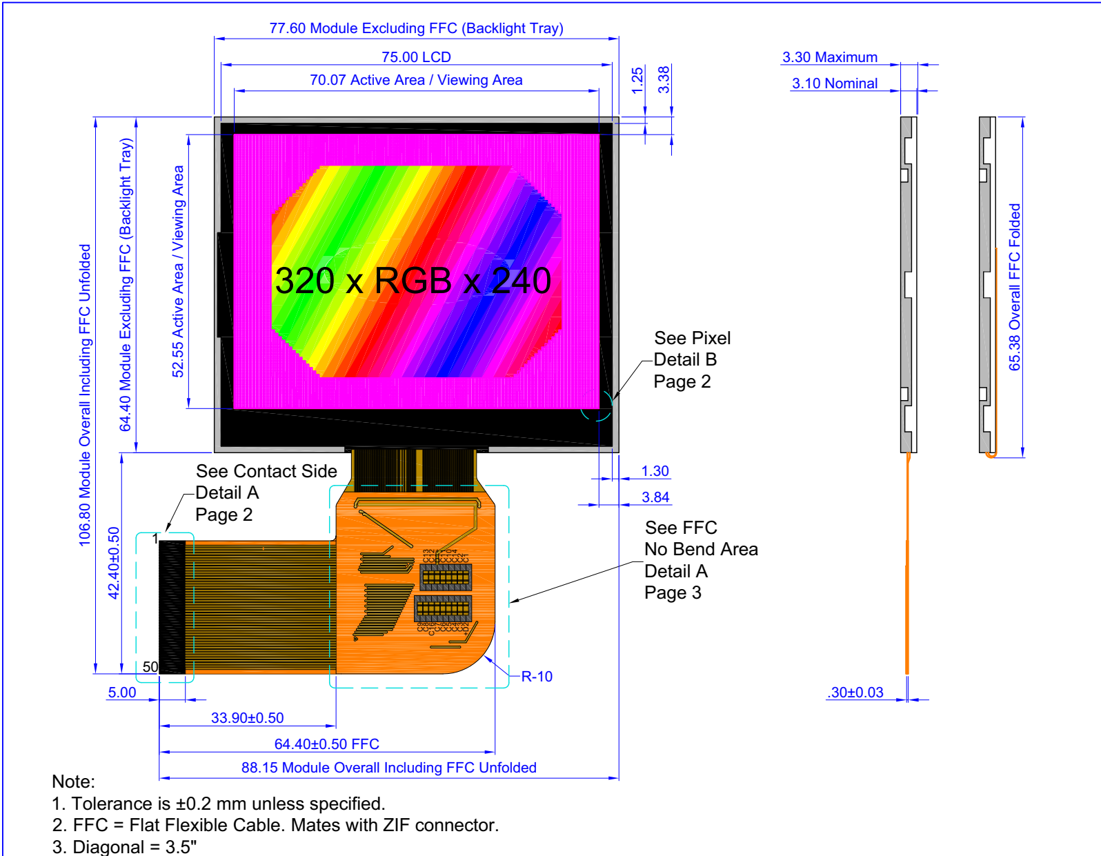
Figure 1. Module Outline Drawings (3 pages)
