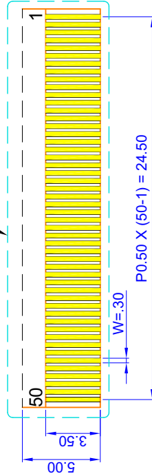
Contact Side Detail A
