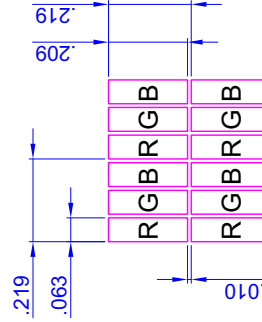
Pixel Detail B
