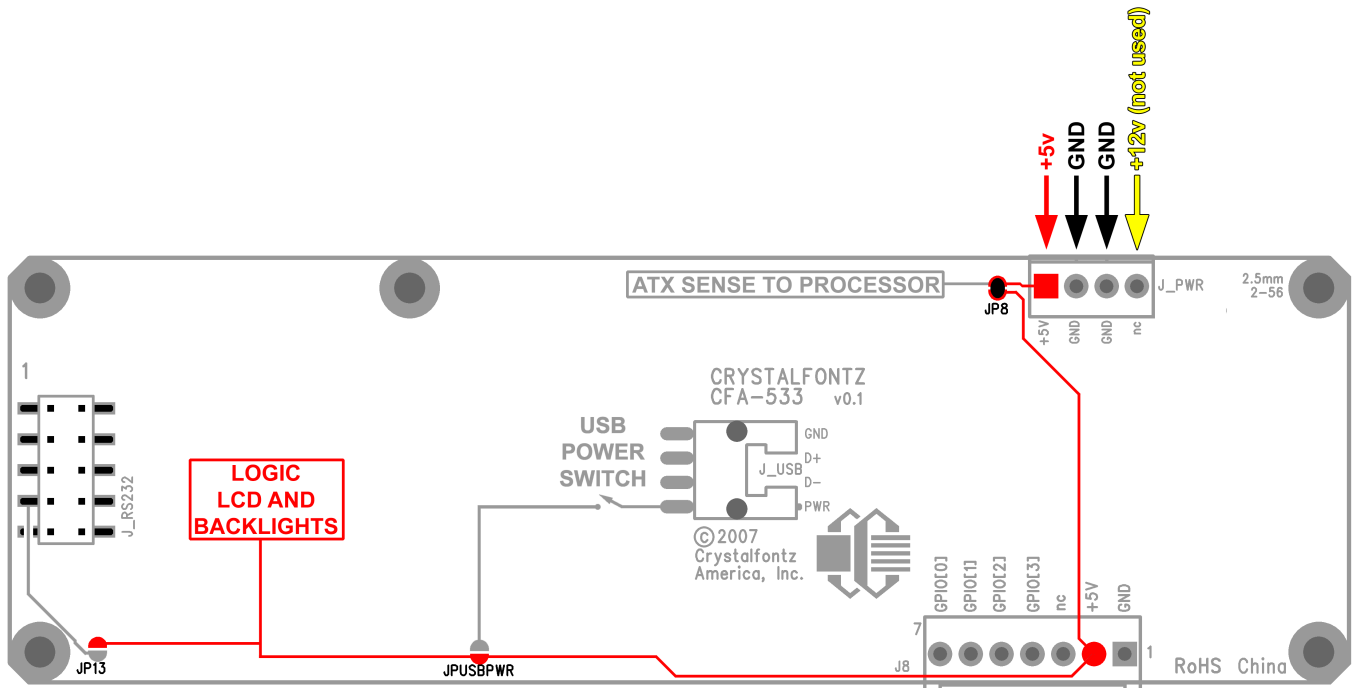
Figure 6. CFA533-YYH-KS Connection for Standard 3 1/2-inch Floppy™
