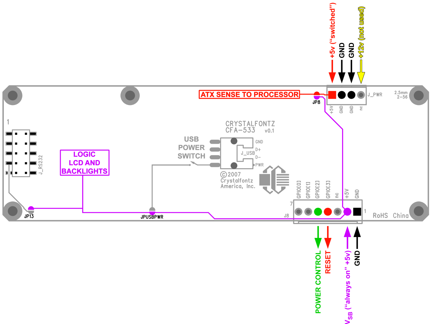
Figure 8. CFA533-YYH-KS ATX Power Supply and Control Connections
