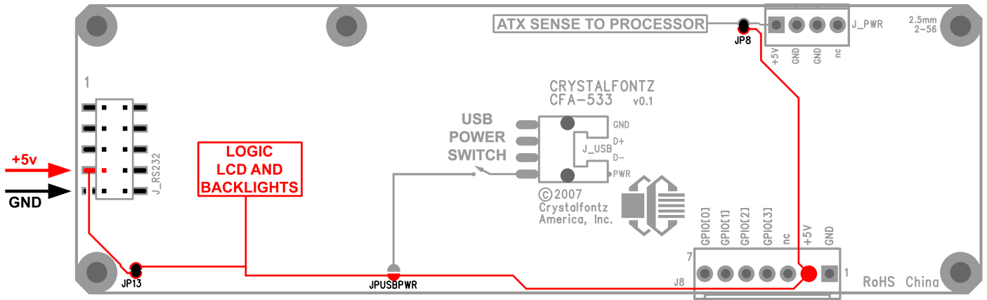
Figure 7. CFA533-YYH-KS RS-232 Power Connection
