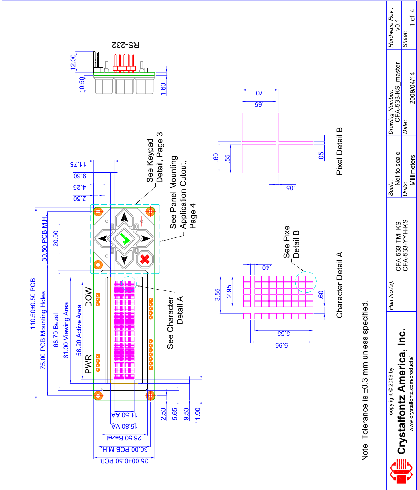
Figure 1. CFA533-YYH-KS Module Outline Drawing (two pages)
