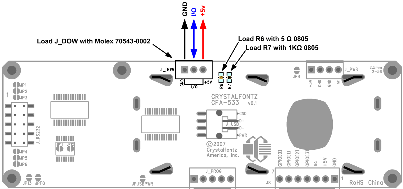
Figure 11. CFA533-YYH-KS Connection for Dallas Semiconductor 1-Wire (DOW) Devices
