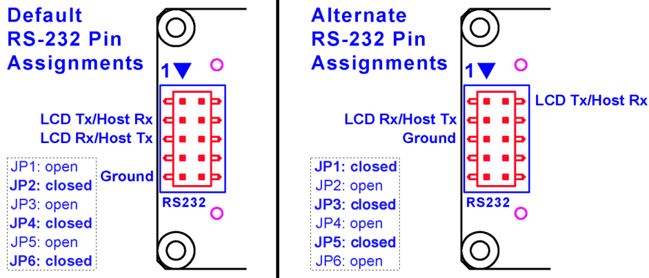
Figure 9. CFA533-YYH-KS Default and Alternate Pin Assignments
