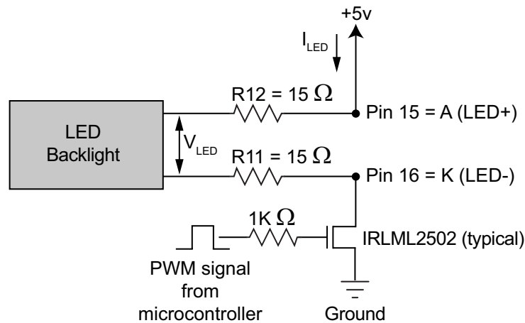
Figure 8. Example of LED Backlight Connections for PWM Dimming
