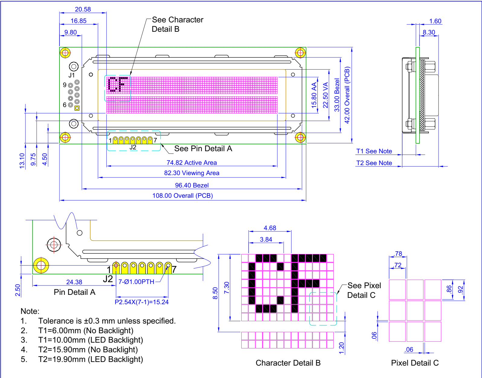
Figure 1. Module Outline Drawings (two pages)
