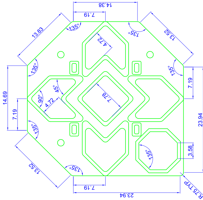
Keypad Detail
